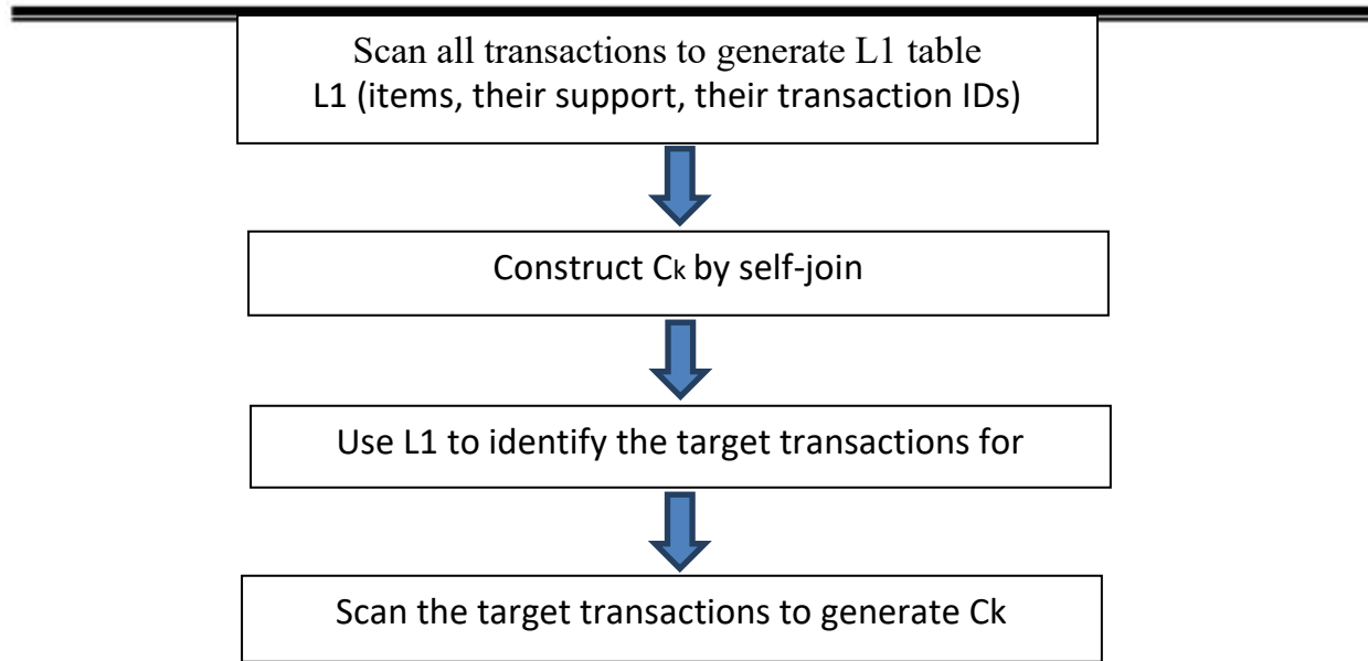
Figure 2: Steps for Ck generation
