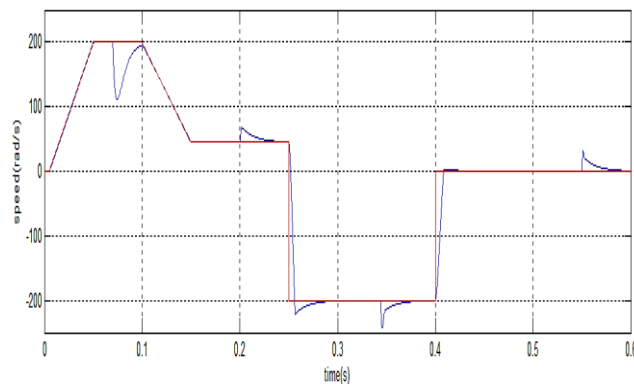
Figure 13: output speed of the large signal simulation
