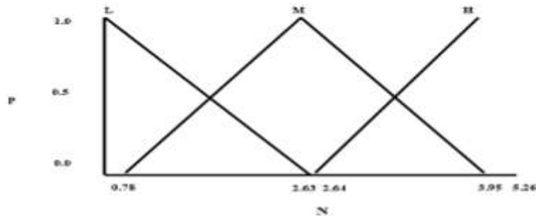
Figure 2. Membership functions for ROC
