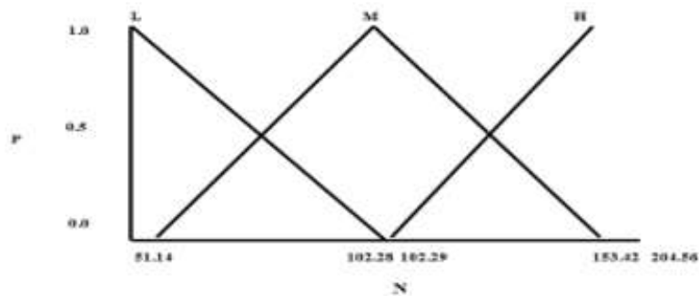
Figure 4. Membership Functions for CTR
