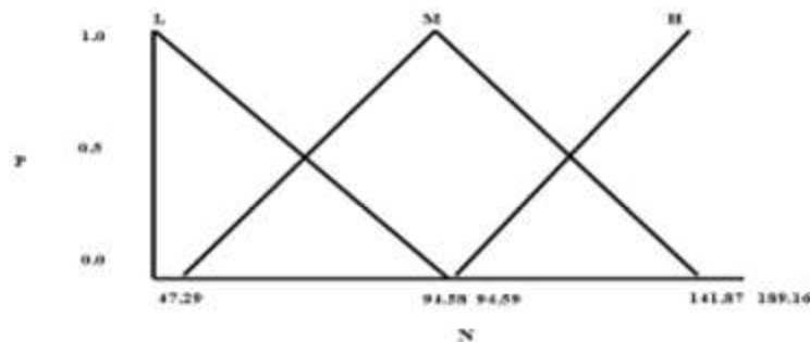
Fig. 7. Membership Functions for DTR
